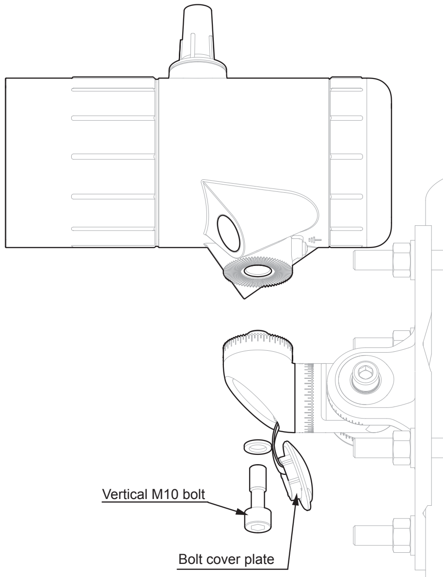
Figure 16. Detector attachment
