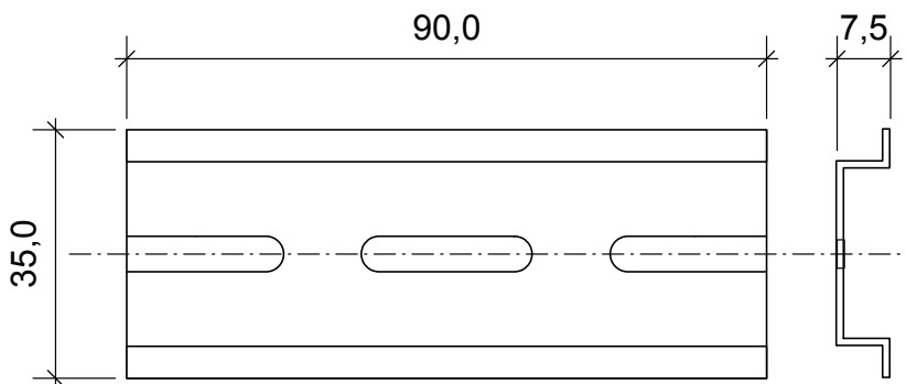
Mounting rail standard (P/N 9602.0050.10.03)
