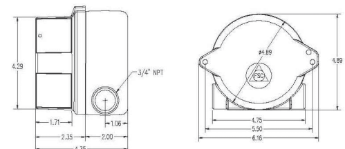
General Dimensions Side and Back Views (All Dimensions in Inches)
